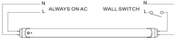
EMERGENCY LED tube wiring schematic
